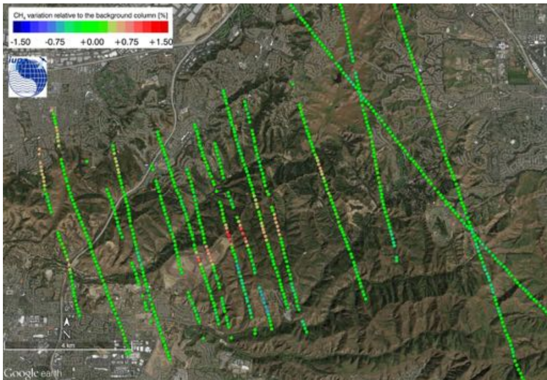
Figure 106: Normalized column averaged dry air mole fraction of CH 4 of the MAMAP remote sensing sounding of the Olinda Alpha Landfill on 2014-09-03.
