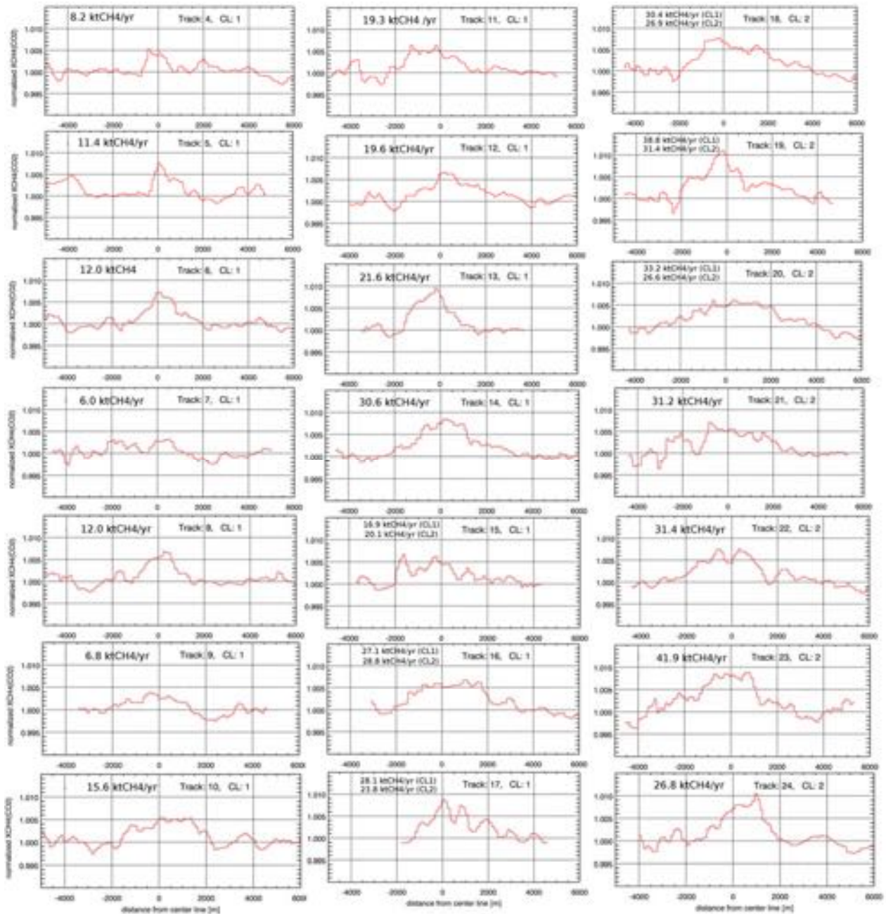
Figure 41: Cross sections of tracks 4 to 24 (to be continued in Figure 42) of the normalized column averaged dry air mole fraction of CH 4 of the MAMAP remote sensing measurements at the Kern Front and Kern River Oil Field on 2014-09-01. The plume limits are +3000 m and the normalization limits are -5000 m to -2000 m and +3000 m to +5000 m (compare to Section 9.1.1). The limits for track 5 and track 17 are slightly narrower due to an obvious offset of the plume, which is caused by the increased XCH 4 (CO 2 ) at around +4000 m, and a very short track, respectively. Each cross section contains labels for the estimated flux and the corresponding center line 1 (northern part) or 2 (southern part). At the transition zone of the wind turn (track 15 to 20), fluxes are given for both center lines. Negative distances point to the south-west and positive distances point to the north-east of the oil field. Wind information from KBFL was used to account for temporal wind variations.
