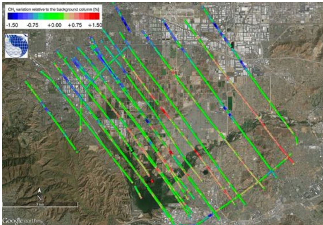
Figure 108: Normalized column averaged dry air mole fraction of CH_4 of the MAMAP remote sensing sounding of the Chino Cattle Ranch / Feed Lot on 2014-09-01.
