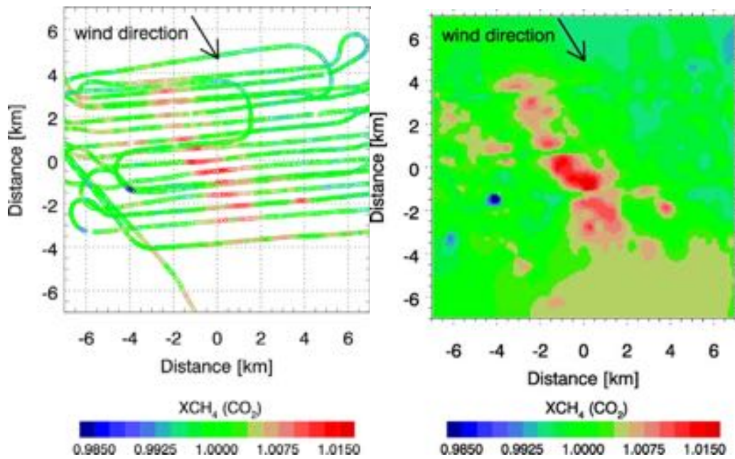
Figure 67: XCH_4(CO_2) retrieved from MAMAP data over Kern Oil Field on 2014-08-26 (left) and interpolated using a Kriging approach (right).
