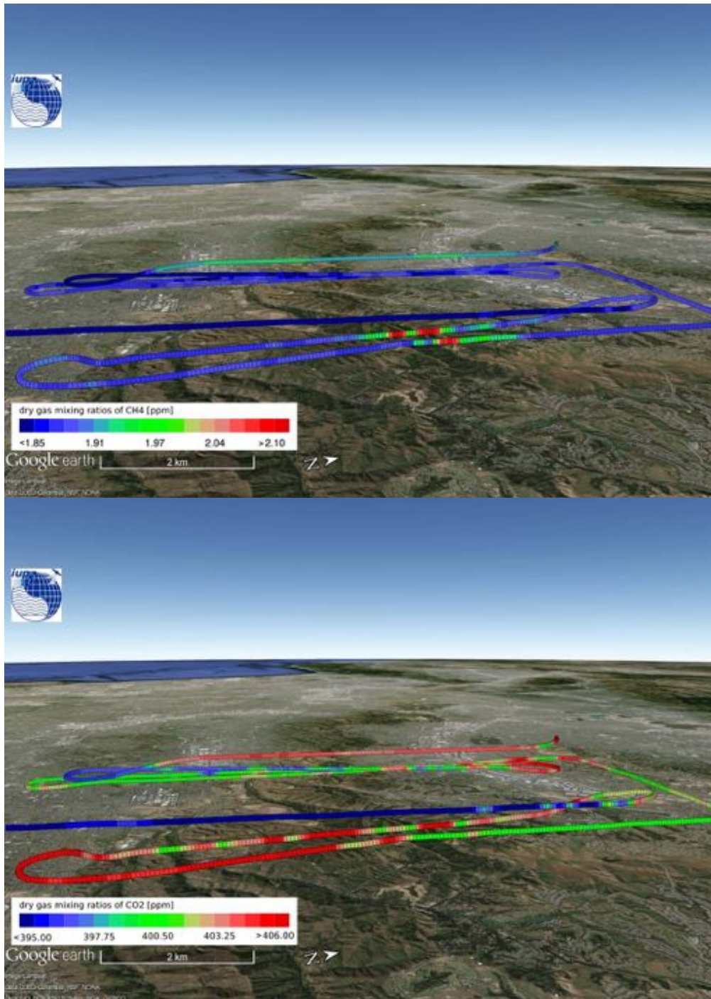
Figure 93: Picarro in-situ measurements of CH 4 (top) and CO 2 (bottom) below remote sensing altitude the Olinda Alpha Landfill on 2014-08-27.
