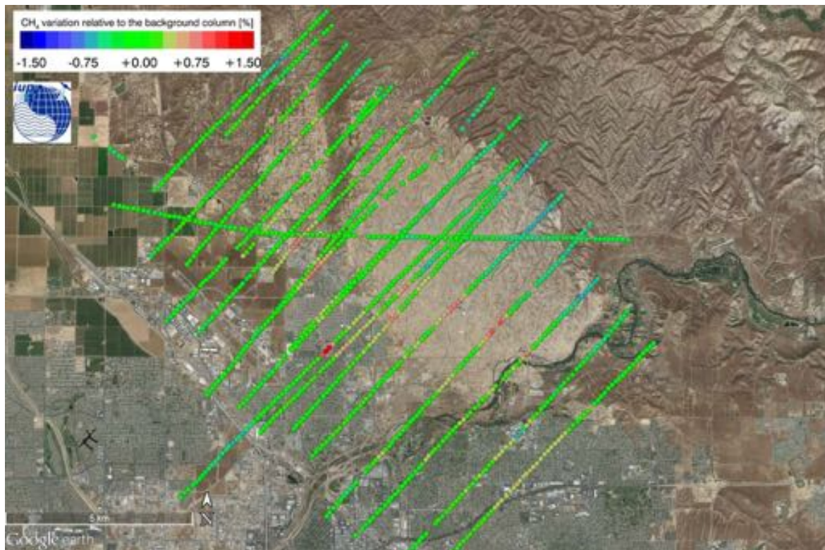
Figure 74: Normalized column averaged dry air mole fraction of CH_4 of the MAMAP remote sensing sounding of the Kern River and Kern Front Oil Field on 2014-06-03.
