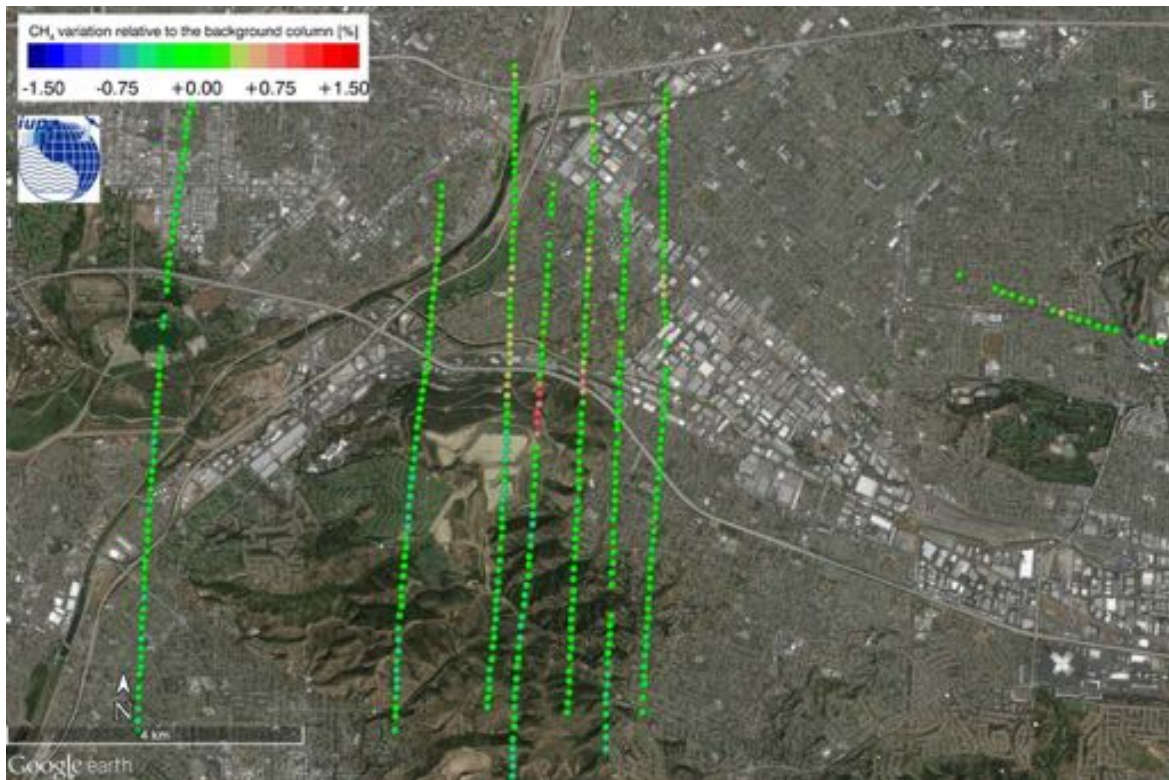
Figure 78: Normalized column averaged dry air mole fraction of CH_4 of the MAMAP remote sensing sounding of the Puente Hills Landfill on 2014-06-12.
