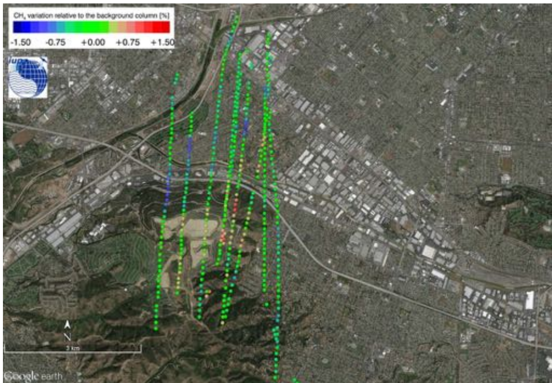
Figure 96: Normalized column averaged dry air mole fraction of CH_4 of the MAMAP remote sensing sounding of the Puente Hills Landfill on 2014-08-28.
