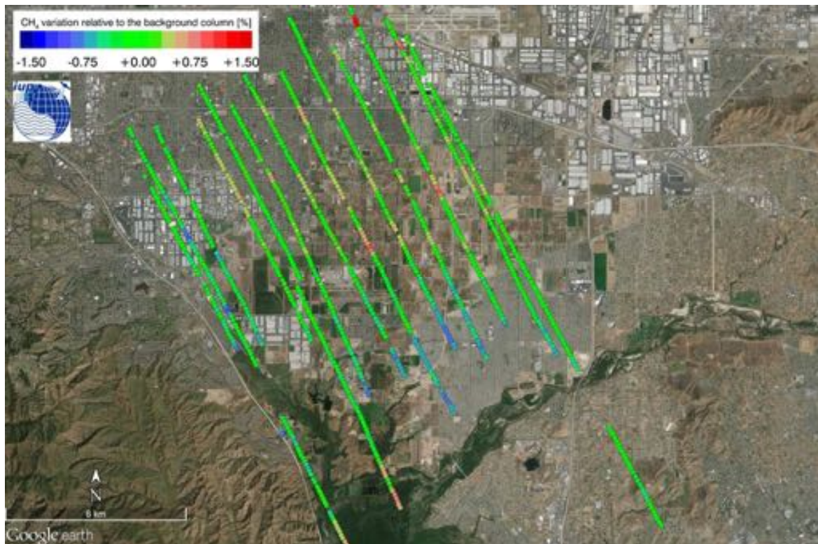
Figure 79: Normalized column averaged dry air mole fraction of CH_4 of the MAMAP remote sensing sounding of the Chino Cattle Ranch / Feed Lot on 2014-06-12.
