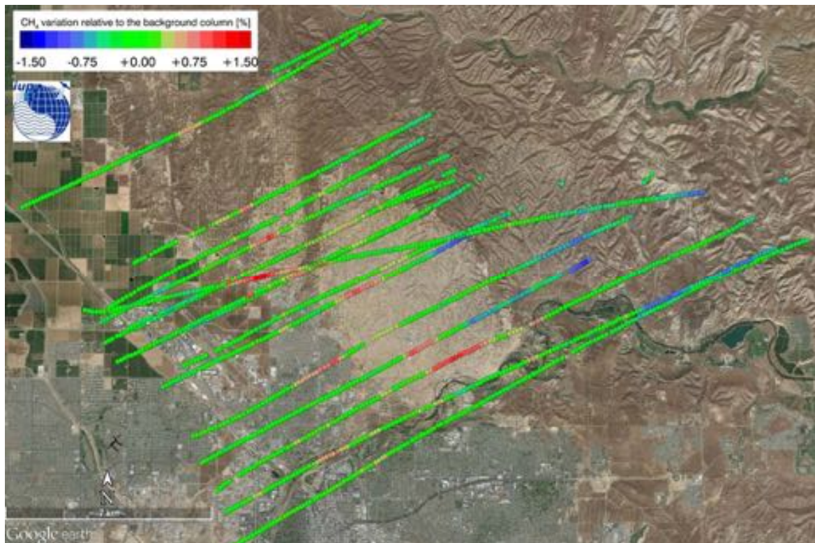
Figure 76: Normalized column averaged dry air mole fraction of CH_4 of the MAMAP remote sensing sounding of the Kern River and Kern Front Oil Field on 2014-06-09.
