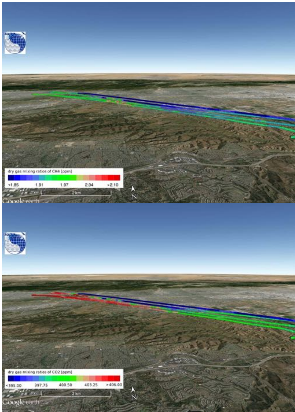
Figure 107: Picarro in-situ measurements of \text{CH}_4 (top) and \text{CO}_2 (bottom) below remote sensing altitude the Olinda Alpha Landfill on 2014-09-03.
