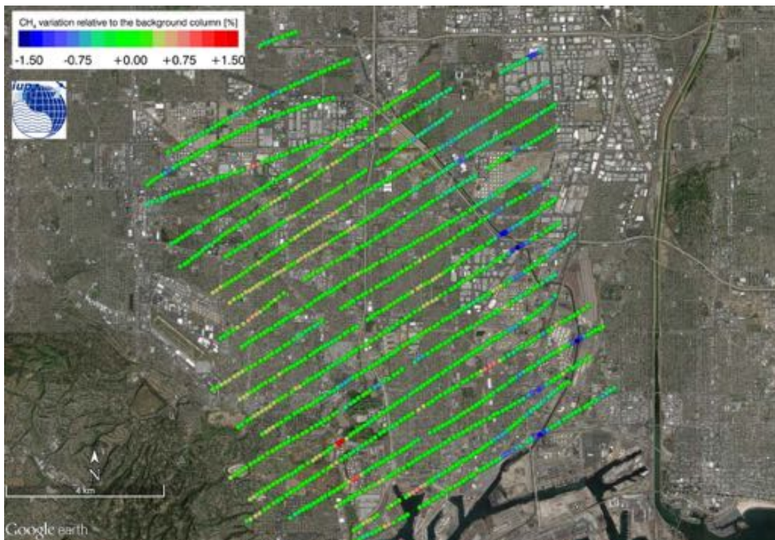
Figure 98: Normalized column averaged dry air mole fraction of CH_4 of the MAMAP remote sensing sounding of the Carson Refinery and Tesoro Refinery on 2014-08-29.
