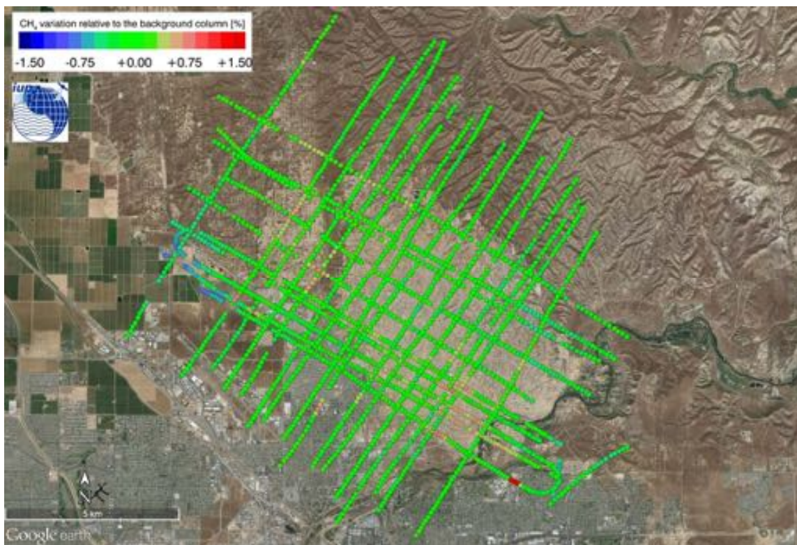
Figure 83: Normalized column averaged dry air mole fraction of CH_4 of the MAMAP remote sensing sounding of the Kern River and Kern Front Oil Field on 2014-08-21.
