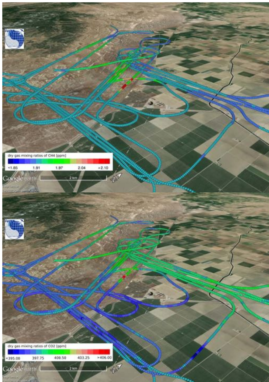
Figure 73: Picarro in-situ measurements of CH 4 (top) and CO 2 (bottom) below remote sensing altitude of Harris Ranch on 2014-05-30.
