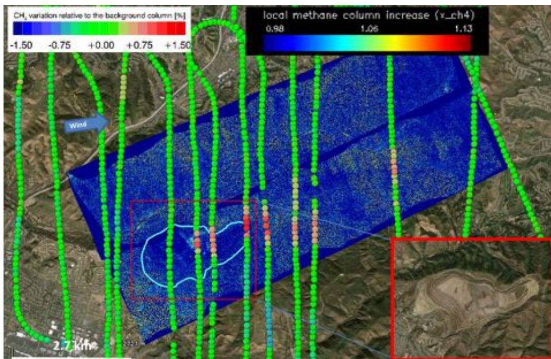
Figure 64: MAMAP and AVIRIS-NG measurements performed contemporaneously on 2014-09-03. The MAMAP data was collected between 20:30-21:15 UTC. AVIRIS-NG overflights shown in the plot were measured at 20:59 UTC and 21:10 UTC, respectively.
