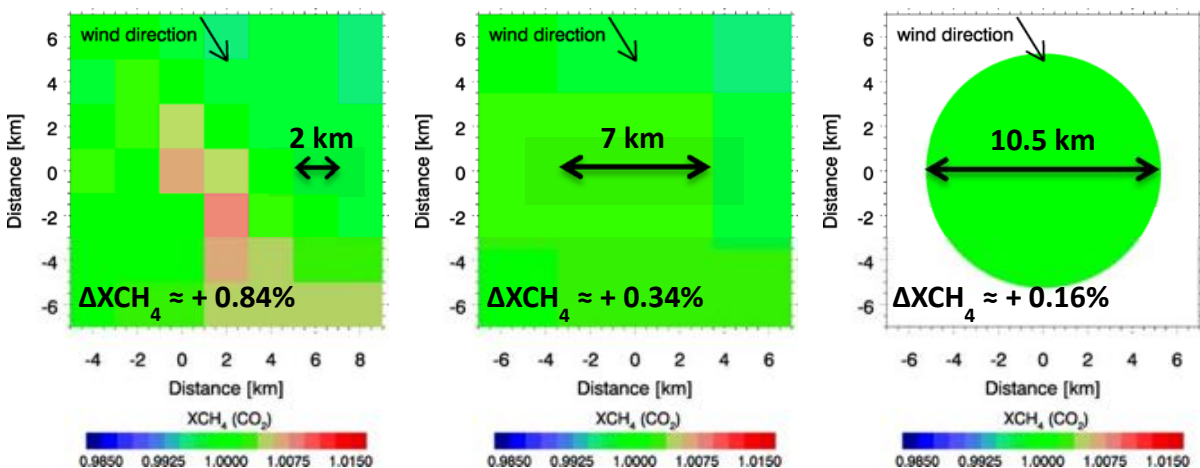
Figure 68: MAMAP retrieved XCH_4(CO_2) regridded to CarbonSat resolution (left), Sentinel-5 Precursor resolution (centre) and GOSAT resolution (right).
