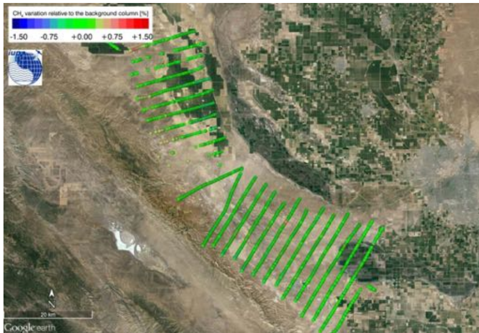
Figure 85: Normalized column averaged dry air mole fraction of CH 4 of the MAMAP remote sensing sounding of the Midway Sunset Oil Field; Elk Hills Oil Field; North Belridge and South Belridge Oil Field; Buena Vista Oil Field on 2014-08-23.
