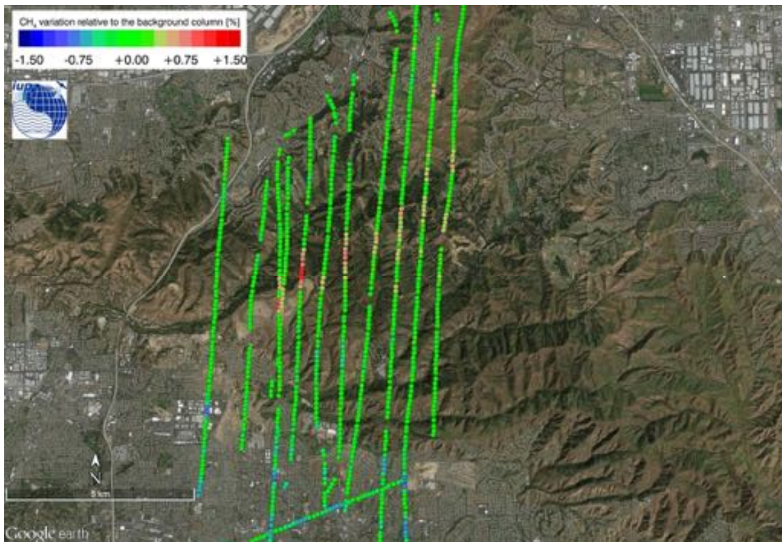
Figure 94: Normalized column averaged dry air mole fraction of CH_4 of the MAMAP remote sensing sounding of the Olinda Alpha Landfill on 2014-08-28.
