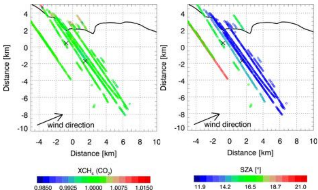
Figure 55: The left plot shows the unsmoothed \text{XCH}_4 data normalized by a regional mean. The corresponding solar zenith angle (SZA) for each data point is shown on the right.
