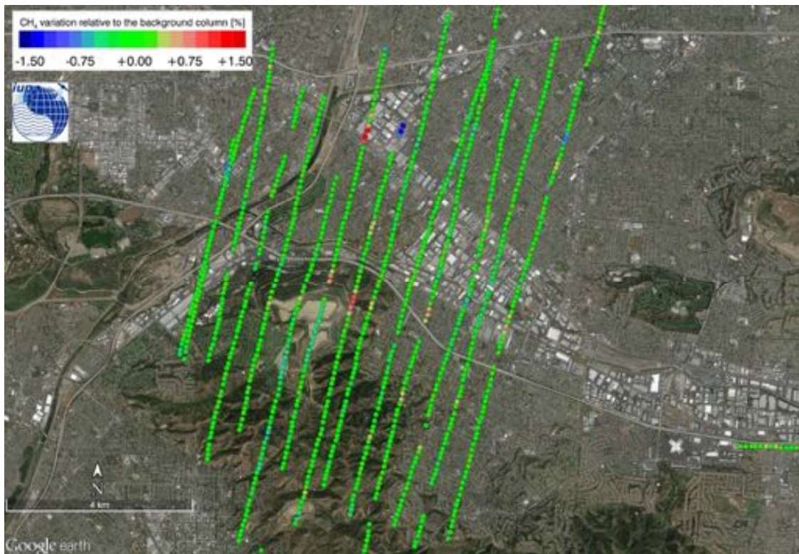
Figure 90: Normalized column averaged dry air mole fraction of CH_4 of the MAMAP remote sensing sounding of the Puente Hills Landfill on 2014-08-27.
