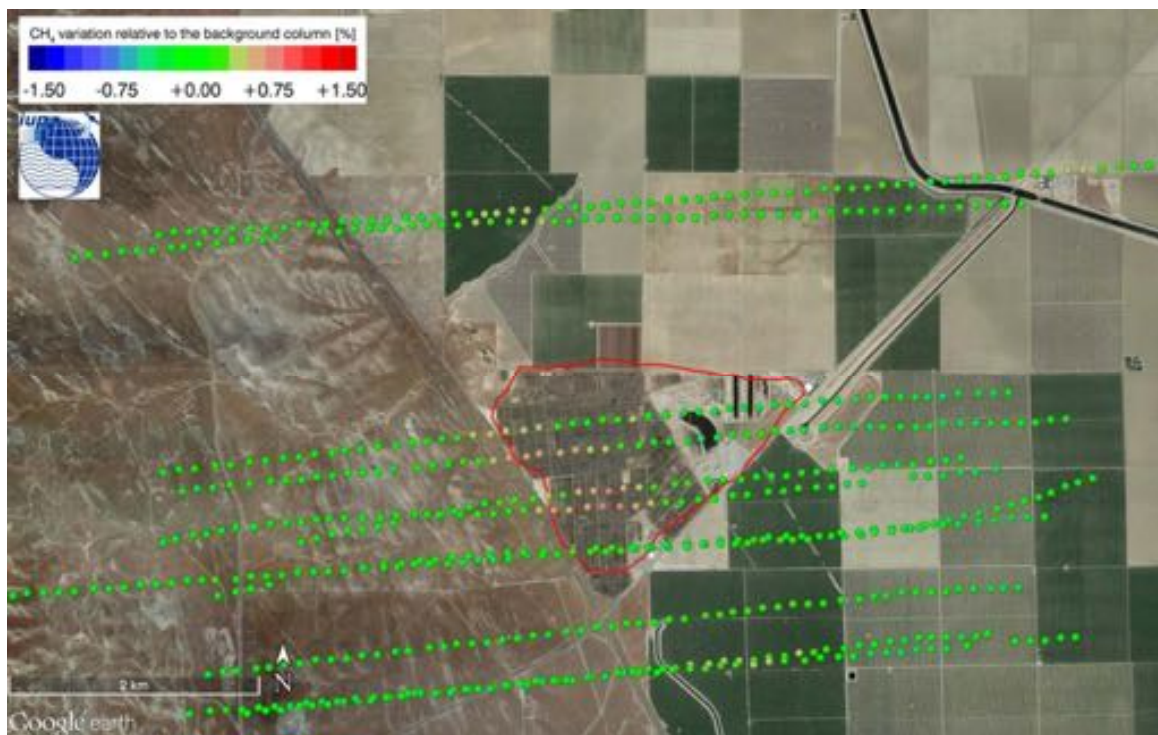
Figure 72: Normalized column averaged dry air mole fraction of CH_4 of the MAMAP remote sensing sounding of Harris Ranch (encircled by the red solid line) on 2014-05-30.
