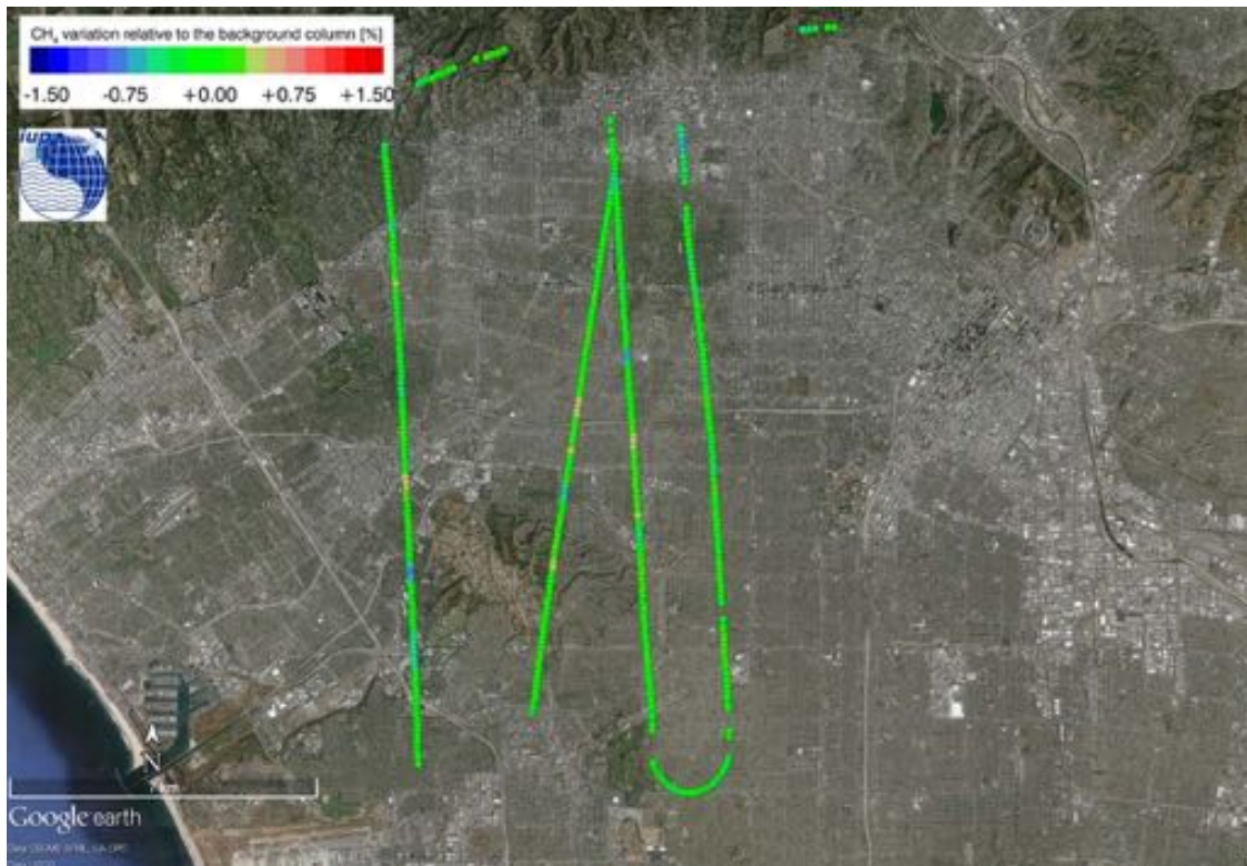
Figure 88: Normalized column averaged dry air mole fraction of CH_4 of the MAMAP remote sensing sounding of the La Brea Tar Pits and the Baldwin Hills Oil Field on 2014-08-27.
