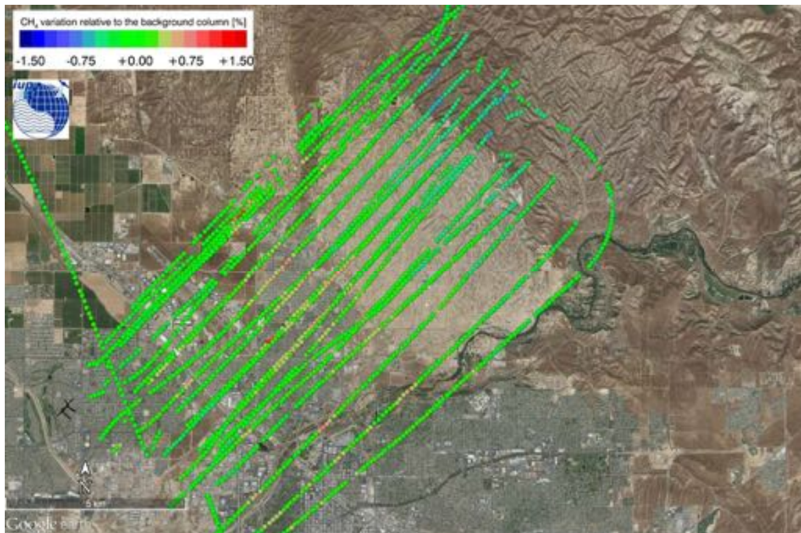
Figure 81: Normalized column averaged dry air mole fraction of CH_4 of the MAMAP remote sensing sounding of the Kern River and Kern Front Oil Field on 2014-06-13.
