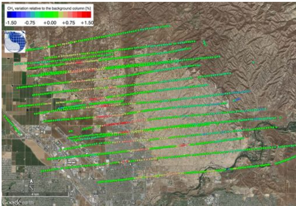
Figure 86: Normalized column averaged dry air mole fraction of CH_4 of the MAMAP remote sensing sounding of the Kern River and Kern Front Oil Field on 2014-08-26.
