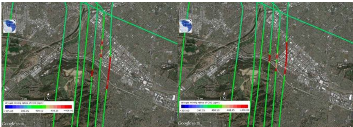
Figure 25: Picarro in-situ measurements of CO_2 at remote sensing altitude over the Puente Hills Landfill on 2014-06-12. Left: Original data set. Right: By 16 s corrected data set.
