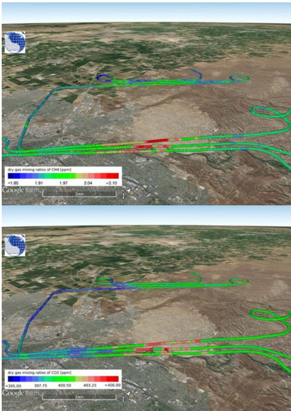
Figure 75: Picarro in-situ measurements of \text{CH}_4 (top) and \text{CO}_2 (bottom) below remote sensing altitude of the Kern River and Kern Front Oil Field on 2014-06-03.
