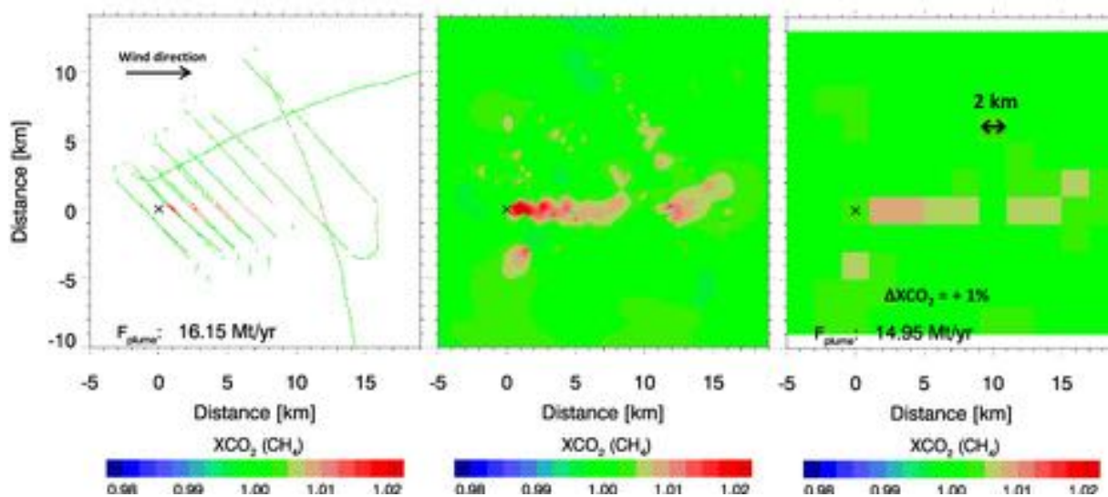
Figure 69: Similar to Figure 70 and Figure 71 but for XCO_2(CH_4) for the coal fired power plant Weisweiler with an emission rate of \sim 15 MtCO 2 /yr for the time of the overflight. Data acquired on 2012-08-18.
