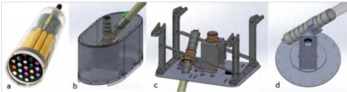
FIGURE 29 a) C-AIR or C-AERO radiometer (shown in a clear plastic housing for demonstration purposes), b) integration of C-AERO global irradiance and sky radiance in fairing mount, c) C-AERO total radiance and C-AIR nadir radiance in nadir port, and d) C-AIR sky radiance, or 3STAR, for sun tracking from the zenith port. 3STAR is C-AIR sky radiance in sun tracking installation.
