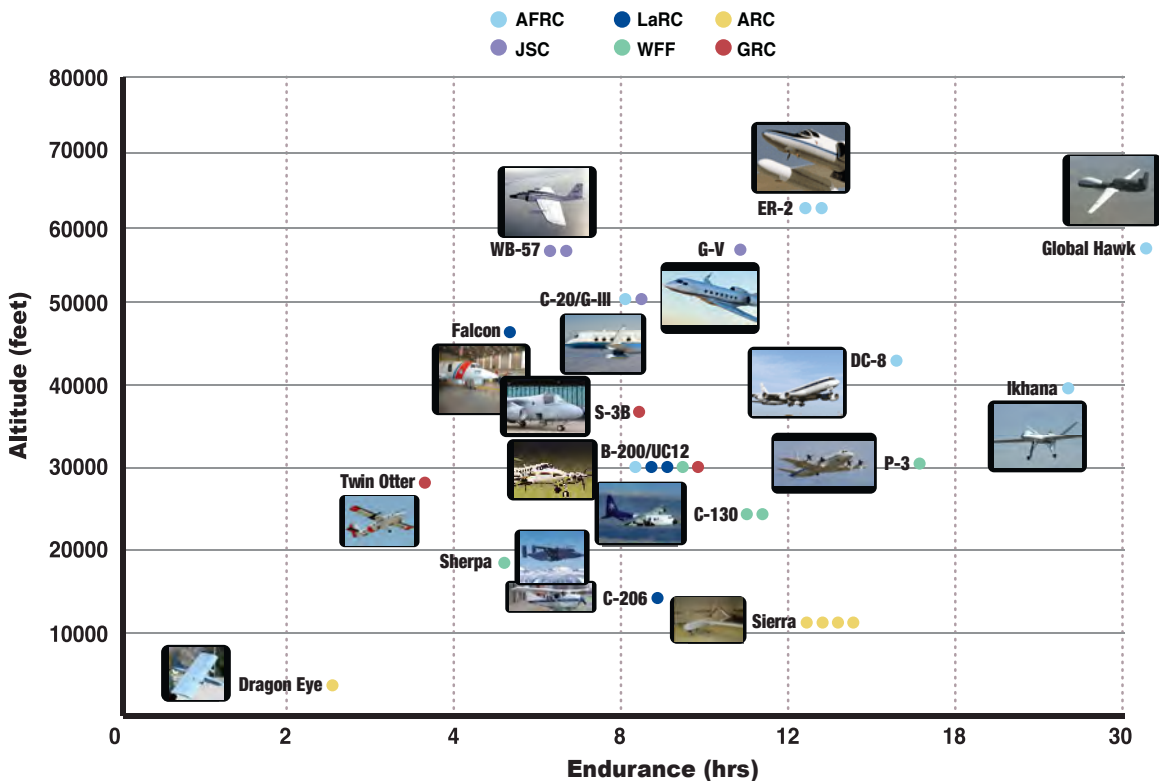
FIGURE 32 NASA Aircraft showing altitude and range capabilities.
