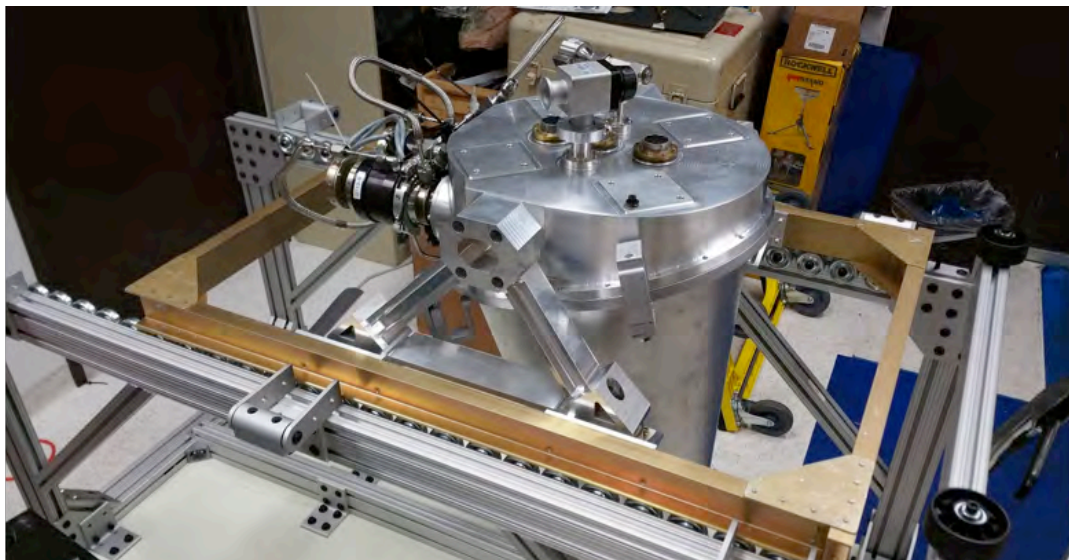
FIGURE 30 New HyTES enclosure mounted in ER-2 installation rail.
