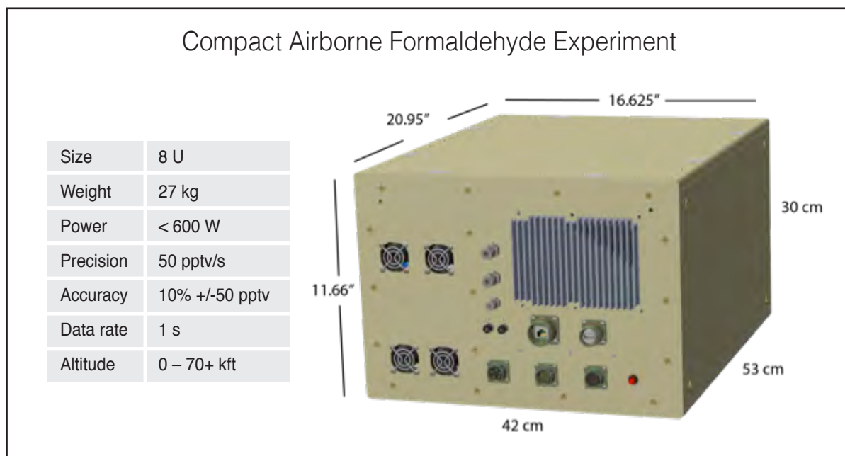
FIGURE 28 Compact Airborne Formaldehyde instrument.
