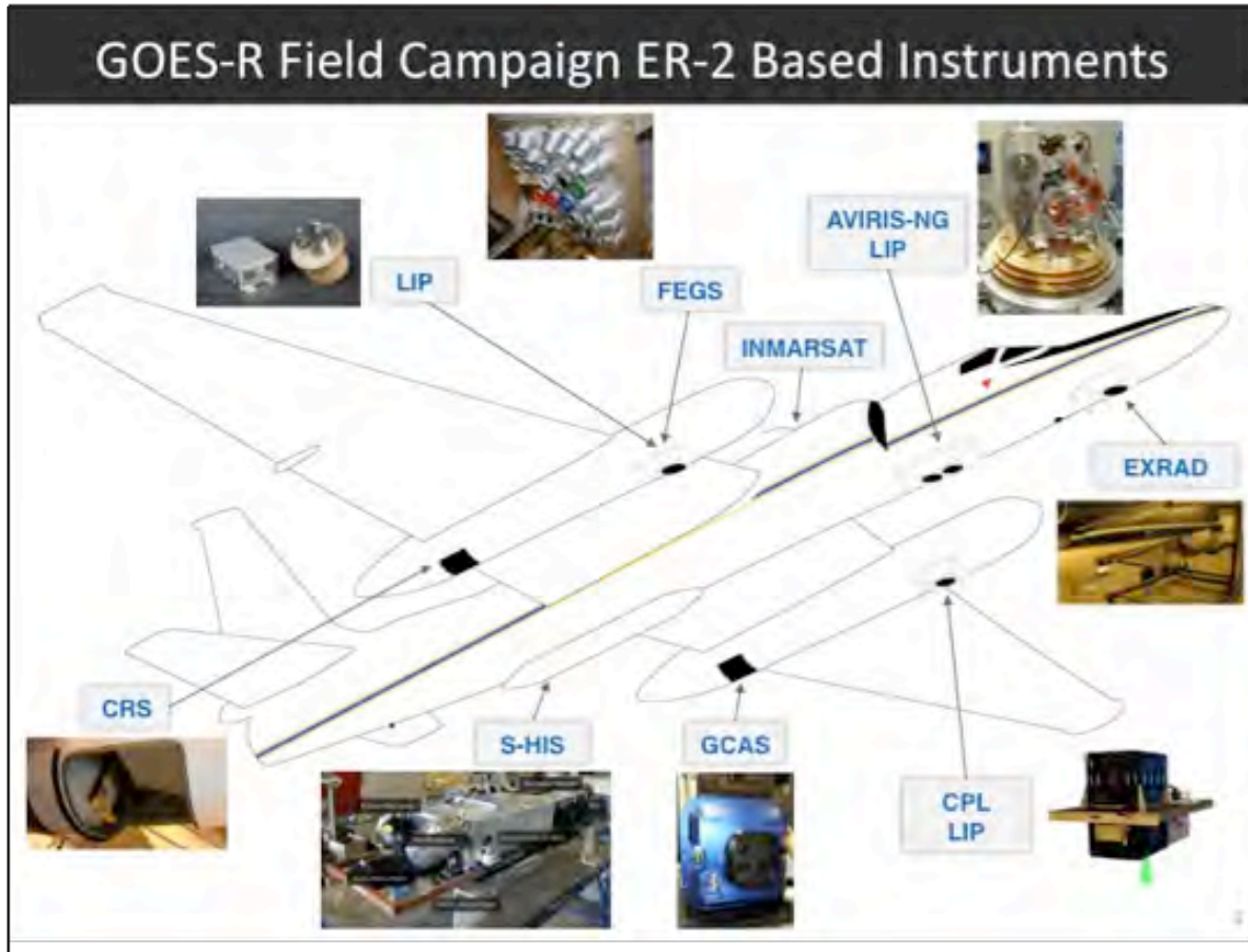
FIGURE 27 GOES-16 Field Campaign ER-2 Based Instruments: Next-Generation Airborne Visible/Infrared Imaging Spectrometer (AVIRISng) & AVIRIS-Classic (AVIRISc); Scanning High-resolution Interferometer Sounder (S-HIS); Fly's Eye GLM Simulator (FECS); Lightning Instrument Package (LIP); Cloud Physics Lidar (CPL); Cloud Radar System (CRS); ER-2 X-band Doppler Radar; GeoCAPE Airborne Simulator (GCAS).
