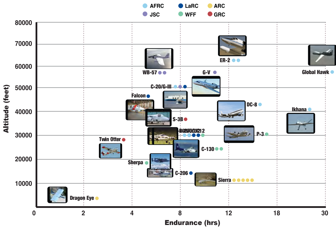
FIGURE 31 NASA Aircraft showing altitude and endurance capabilities.
